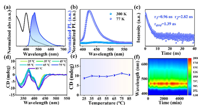
Fig. 2 (a) UV absorption and PL emission spectra of (R-MPEA) 4 AgBiBr 8 NBs. (b) Temperature-dependent PL spectra, (c) time-resolved PL decays spectra, (d) temperature-dependent CD spectra, (e) corresponding CD intensity at CD peaks of 420 nm and (f) PL intensity of (R-MPEA) 4 AgBiBr 8 NBs under ambient conditions with the relative humidity of RH = 65 \pm 5\% .
