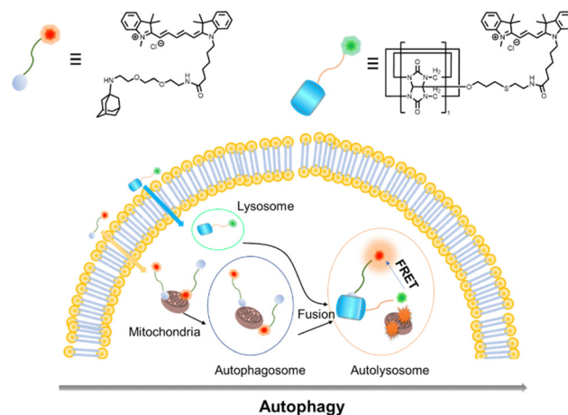
Fig. 9 Chemical structures of \text{CB}[7]\text{-Cy3} and \text{AdA-Cy5} and the emergence of FRET after the fusion of two different organelles through the process of autophagy.
