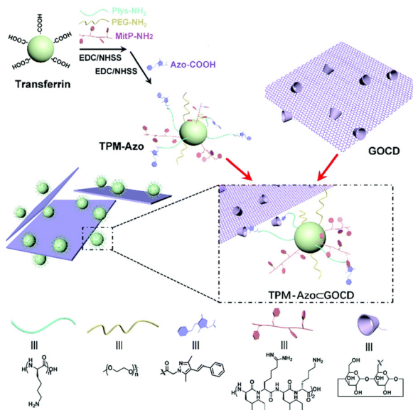
Fig. 20 Synthesis of the TPM-Azo guest, the GOCD host, and the TPM-Azo \subset GOCD host-guest supramolecular nanoassemblies. Reproduced with permission from ref. 114. Copyright 2019 The Royal Society of Chemistry.
