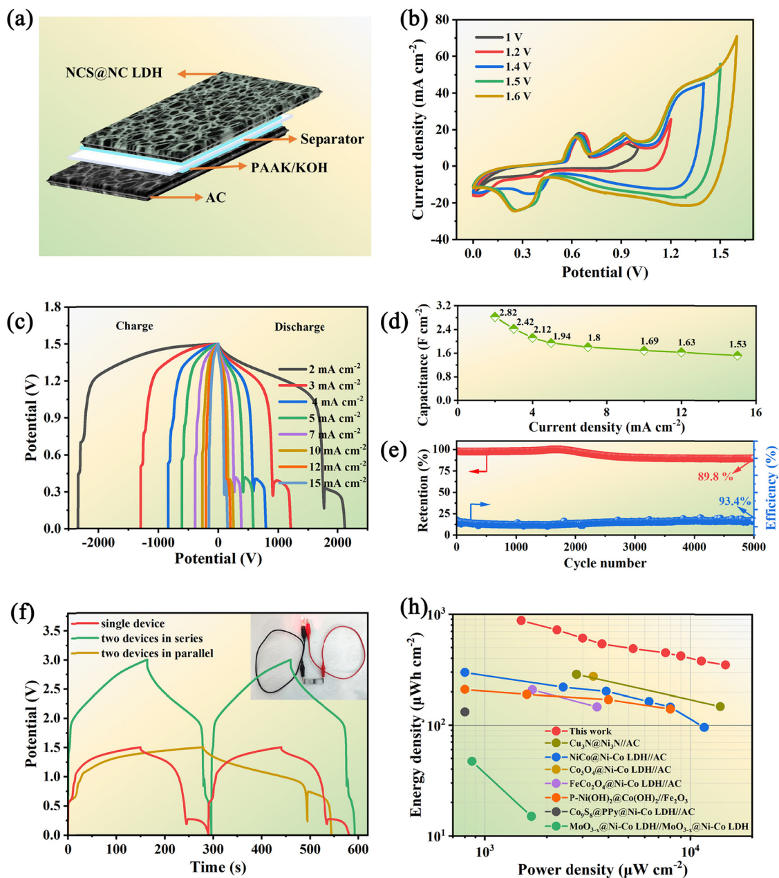
Fig. 7 (a) Schematic diagram of the assembled NCS@NC LDH//AC ASC. (b) CV curves with different potential windows at a scan rate of 10 mV s -1 . (c) GCD curves of the ASC at various current densities. (d) Areal specific capacitance of the ASC device. (e) Capacitance retention and coulombic efficiency after 5000 cycles. (f) GCD curves of two ASC devices connected in parallel and in series at a current density of 15 mA cm -2 . (g) Ragone plot related to the power density and energy density of the ASC in comparison with the literature results.
