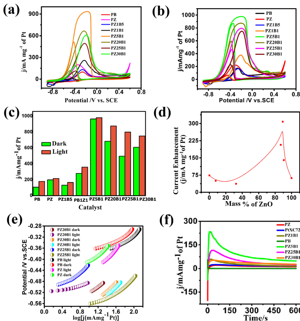
Fig. 7 (a) Cyclic voltammograms of all the constructed electrodes at 50\text{ mV s}^{-1} scan rate in 0.5\text{ M MeOH} + 1\text{ M NaOH} solution in the absence of light. (b) CV of the same electrodes with visible light exposition. (c) The histogram profiles of the current density of the synthesized electrodes with different mass ratios of ZnO and \text{Bi}_2\text{O}_3 . (d) The plot of enhancement of current ( \text{mA mg}^{-1} of Pt) versus mass percentage of ZnO under visible light (e) Tafel plots of PB, PZ, PZ20B1, PZ25B1, and PZ30B1 electrodes achieved from CV experiments in 0.5\text{ M MeOH} + 1\text{ M NaOH} solution operated at 1\text{ mV s}^{-1} scan rate under dark and light illumination. (f) Chronoamperometric curves of the constructed electrodes immersed in 0.5\text{ M MeOH} + 1\text{ M NaOH} solution, executed at -0.3\text{ V} potential up to 600 s under visible light.
