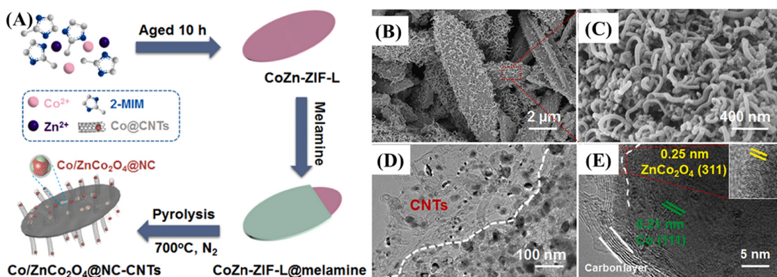
Fig. 20 (A) Schematic synthesis process of the \text{Co/ZnCo}_2\text{O}_4@NC-CNT electrocatalyst. (B and C) SEM images, (D) TEM image, and (E) HRTEM image of the as-prepared \text{Co/ZnCo}_2\text{O}_4@NC-CNTs . Reproduced with permission. 255 Copyright © 2020 Elsevier Ltd. All rights reserved.
