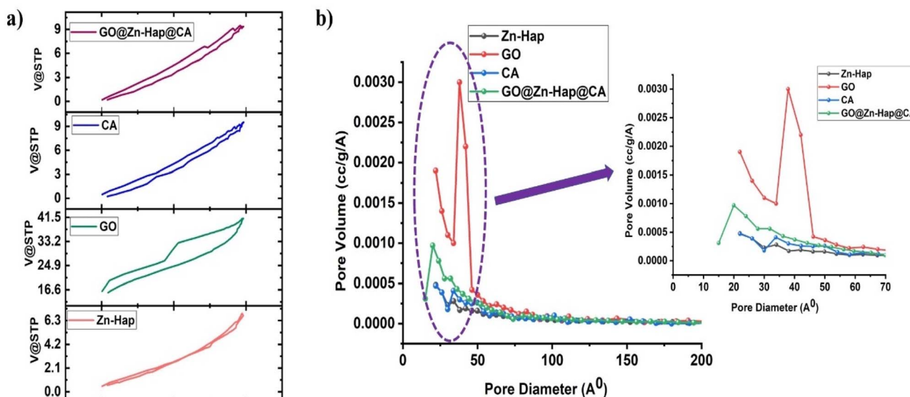
Fig. 5 (a) N_2 adsorption-desorption isotherms, (b) BJH adsorption pore size distribution for GO, Zn-Hap, CA membrane and GO@Zn-Hap@CA.
