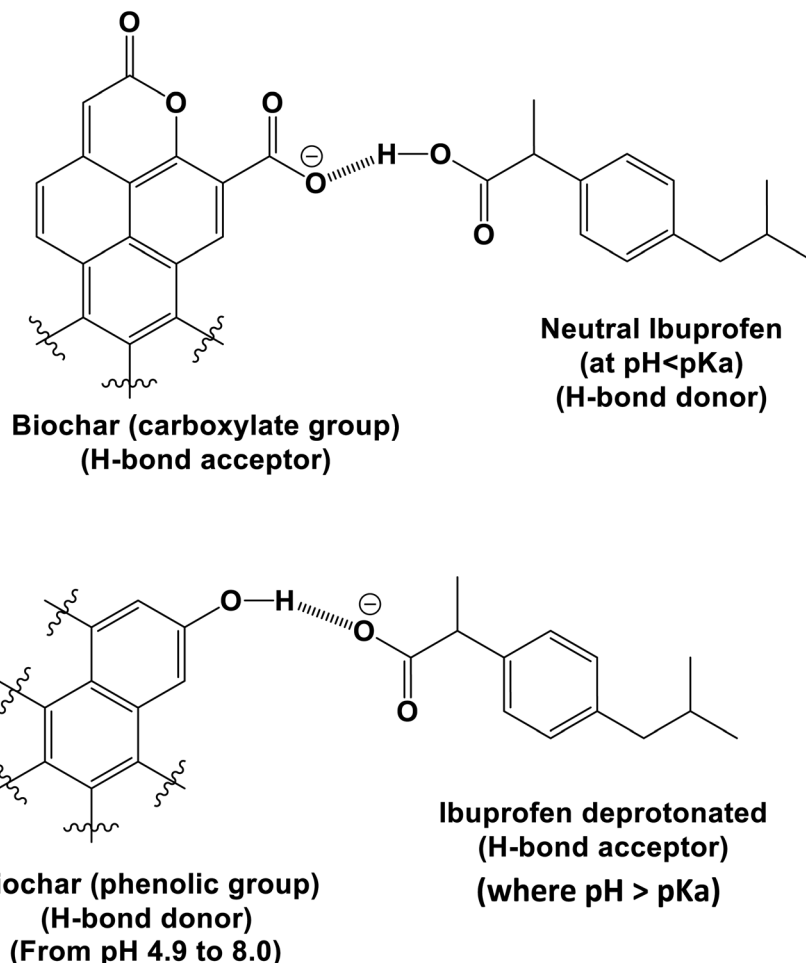
Scheme 4 WSBC hydrogen bonding from ibuprofen ( \text{pH} < \text{pK}_a ) and to ibuprofen ( \text{pH} > \text{pK}_a ).
