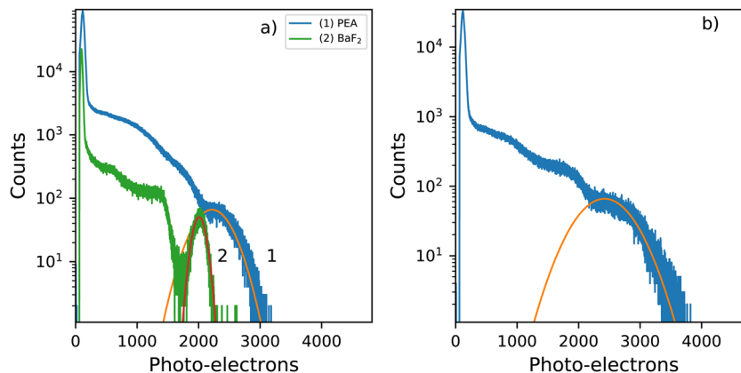
Fig. 8 Pulse height spectra recorded using a 137 Cs \gamma -source and a PMT as detector (a) Small, similar sized, PEA 2 PbBr 4 and BaF 2 . (2 mm \times 1 mm \times 0.3 mm) (b) Large PEA 2 PbBr 4 crystal (8 mm \times 5 mm \times 1 mm).
