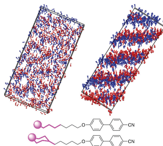
Fig. 10 Snapshots of the simulations of 8OBC at 75 ns (left) and 9 at 646 ns (right) showing the terminal alkyl carbon atoms from C_4 onwards, as shown in bold on the structures (bottom); the terminal carbon atoms are represented by spheres to assist orientation. Up and down molecules are coloured red and blue, respectively, and the simulation boxes are oriented with the layer normal vector vertical.
