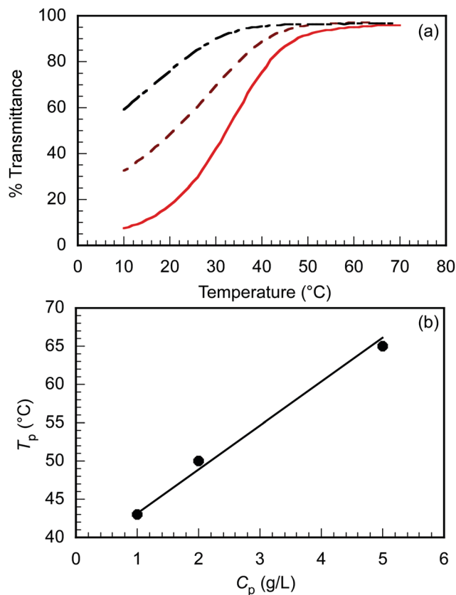
Fig. 2 (a) Percent transmittance (%T) of EUM in PBS at various C_p = 1.0 (---), 2.0 (---), and 5.0 \text{g L}^{-1} (—) as a function of temperature with the cooling process, and (b) phase transition temperature ( T_p ) of EUM in PBS as a function of C_p .
