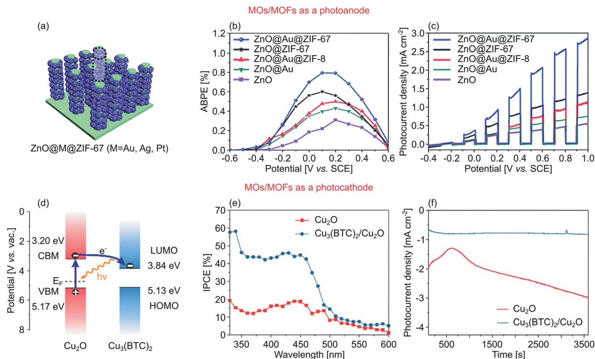
Fig. 12 (a) An artist's rendition of \text{ZnO}@M@ZIF-67 ( M = \text{Au}, \text{Ag}, \text{Pt} ) photoanode for PEC water splitting, and (c) polarization curves of \text{ZnO} , \text{ZnO}@Au , \text{ZnO}@ZIF-67 , \text{ZnO}@Au@ZIF-67 , and \text{ZnO}@Au@ZIF-8 heterostructures under chopped-light irradiation. (d) Schematic band diagram of \text{Cu}_2\text{O}/\text{Cu}_3(\text{BTC})_2 heterostructure photocathode. (e) Wavelength-dependent IPCE and (f) I-t curves of the \text{Cu}_2\text{O} and \text{Cu}_2\text{O}/\text{Cu}_3(\text{BTC})_2 . Figures adapted with permission from: (a–c) ref. 190. Copyright 2017 The Royal Society of Chemistry. (d–f) Ref. 233. Copyright 2019 American Chemical Society.
