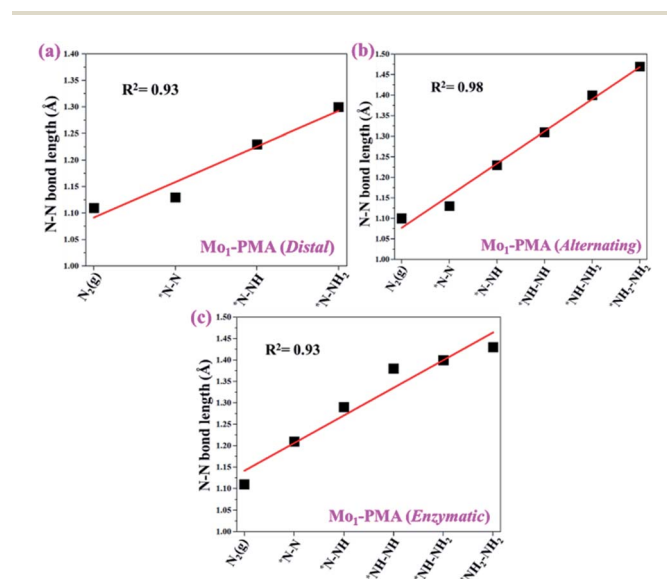
Fig. 12 N–N bond length along (a) distal, (b) alternating, and (c) enzymatic pathways over the \text{Mo}_1/\text{PMA} cluster, respectively. The corresponding bond length values are presented in Table S5.†
