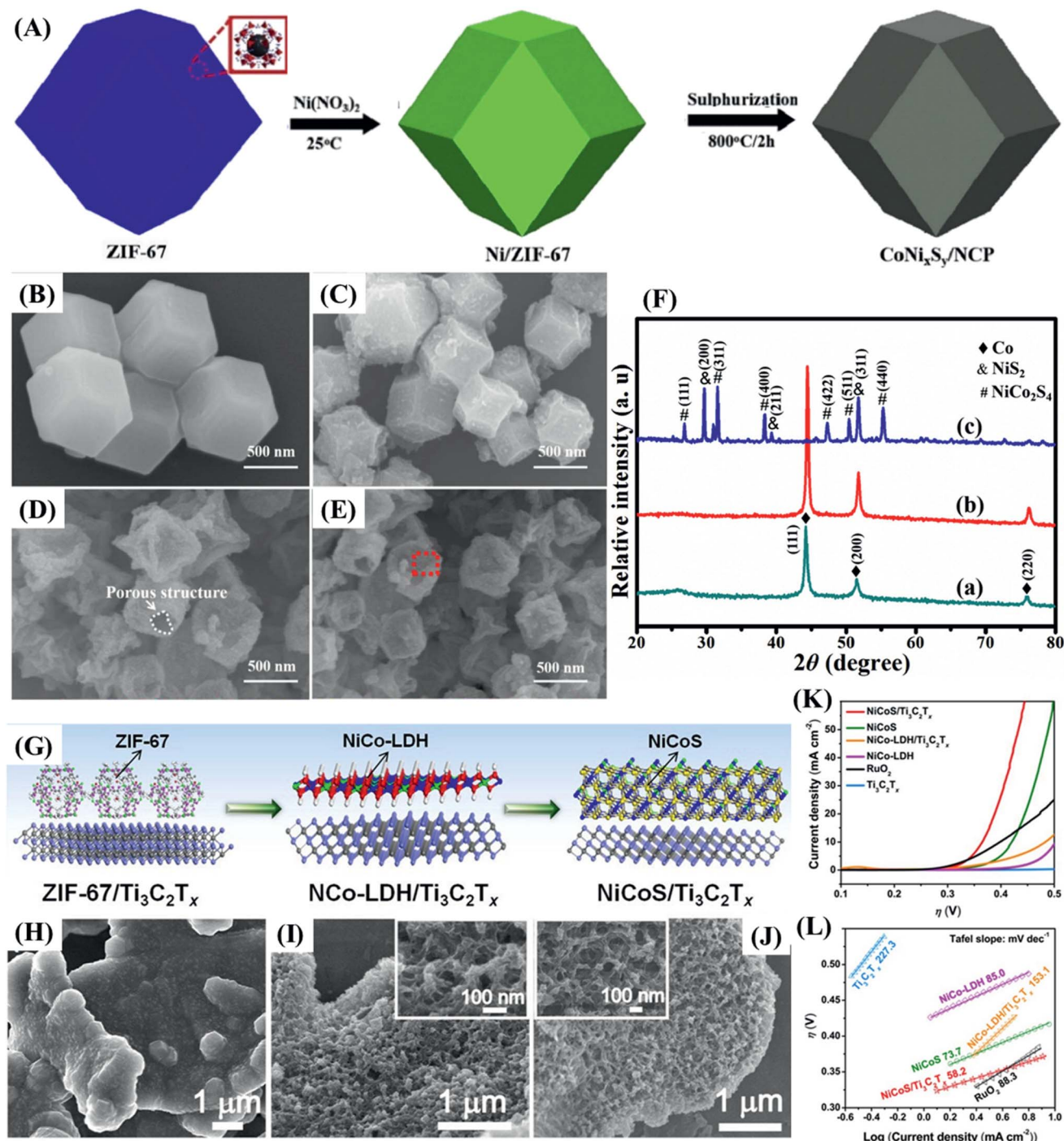
Fig. 22 (A) Scheme showing the fabrication of the \text{CoNi}_x\text{S}_y/\text{NCP} composite. SEM images of (B) ZIF-67, (C) Co/NC, (D) \text{CoNi}_x/\text{NCP} , and (E) \text{CoNi}_x\text{S}_y/\text{NCP} . (F) XRD patterns of (a) Co/NC, (b) \text{CoNi}_x/\text{NCP} , and (c) \text{CoNi}_x\text{S}_y/\text{NCP} . Adapted with permission from ref. 103. Copyright© 2019 Hydrogen Energy Publications LLC. Published by Elsevier Ltd. All rights reserved. (G) Scheme depicting the preparation of \text{NiCoS}/\text{Ti}_3\text{C}_2\text{T}_x . SEM images of (H) ZIF-67/ \text{Ti}_3\text{C}_2\text{T}_x , (I) NiCo-LDH/ \text{Ti}_3\text{C}_2\text{T}_x , and (J) \text{NiCoS}/\text{Ti}_3\text{C}_2\text{T}_x . Inset: the high-magnification SEM images of the samples. (K) LSV curves and (L) Tafel plots of \text{NiCoS}/\text{Ti}_3\text{C}_2\text{T}_x , \text{NiCoS} , \text{NiCo-LDH}/\text{Ti}_3\text{C}_2\text{T}_x , \text{NiCo-LDH} , and \text{RuO}_2 . Reproduced with permission from ref. 104. Copyright© 2018, American Chemical Society.
