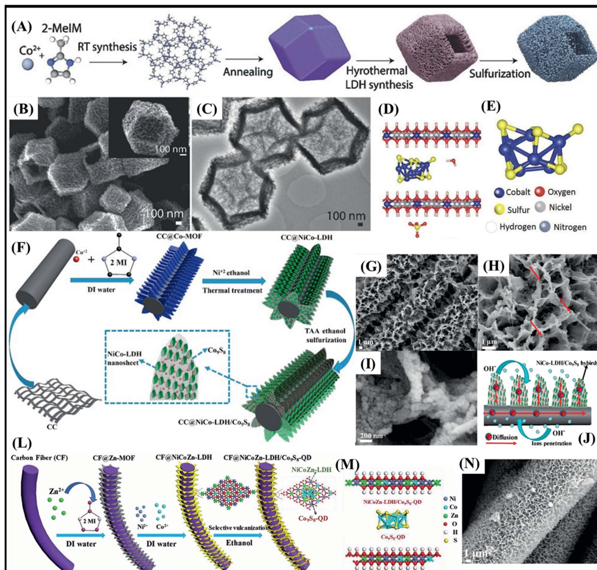
Fig. 12 (A) Scheme illustrating the synthesis of the hollow \text{NiCo-LDH/Co}_9\text{S}_8 hybrid. (B) Panoramic and single (inset) SEM images, and (C) TEM image (g) of \text{NiCo-LDH/Co}_9\text{S}_8 polyhedrons. (D) Optimized structures of \text{NiCo-LDH/Co}_9\text{S}_8 and (E) isolated \text{Co}_9\text{S}_8 . Reproduced with permission. 6 Copyright© 2017 Wiley-VCH Verlag GmbH & Co. KGaA, Weinheim. (F) A schematic showing the fabrication process of the \text{CC@NiCo-LDH/Co}_9\text{S}_8 hybrid nanosheet arrays. (G–I) SEM images of the \text{CC@NiCo-LDH/Co}_9\text{S}_8 hybrid nanosheet arrays. (J) Schematic illustration displaying the merits of the hierarchical \text{CC@NiCo-LDH/Co}_9\text{S}_8 electrode for energy storage. Reproduced with permission. 53 Copyright© 2018. Published by Elsevier B.V. (L) Scheme illustrating the fabrication of the \text{CF@NiCoZn-LDH/Co}_9\text{S}_8\text{-QD} hybrid nanosheet arrays, and (M) its optimized structure. (N) SEM images of \text{CF@NiCoZn-LDH/Co}_9\text{S}_8\text{-QD} hybrid nanosheet arrays. Reproduced with permission. 67 Copyright© 2020 Wiley-VCH Verlag GmbH & Co. KGaA, Weinheim.
