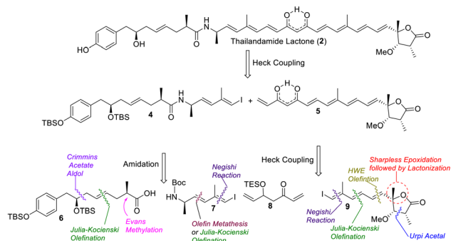
Scheme 1 Retrosynthetic analysis of thailandamide lactone (2).
