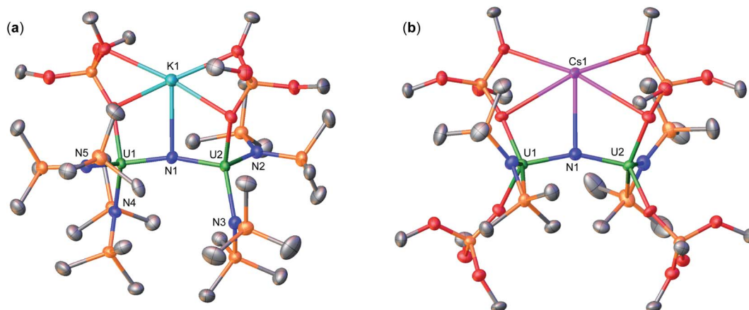
Fig. 1 Molecular structures of (a) [K\{U^{IV}(OSi(O^tBu)_3)(N(SiMe_3)_2)_2\}_2(\mu-N)] , 1 , and (b) [Cs\{U^{IV}(OSi(O^tBu)_3)_2(N(SiMe_3)_2)_2(\mu-N)\}] , 3-Cs , with thermal ellipsoids at drawn at the 50% probability level. Hydrogen atoms and methyl groups on the OSi(O^tBu)_3 ligands have been omitted for clarity.
