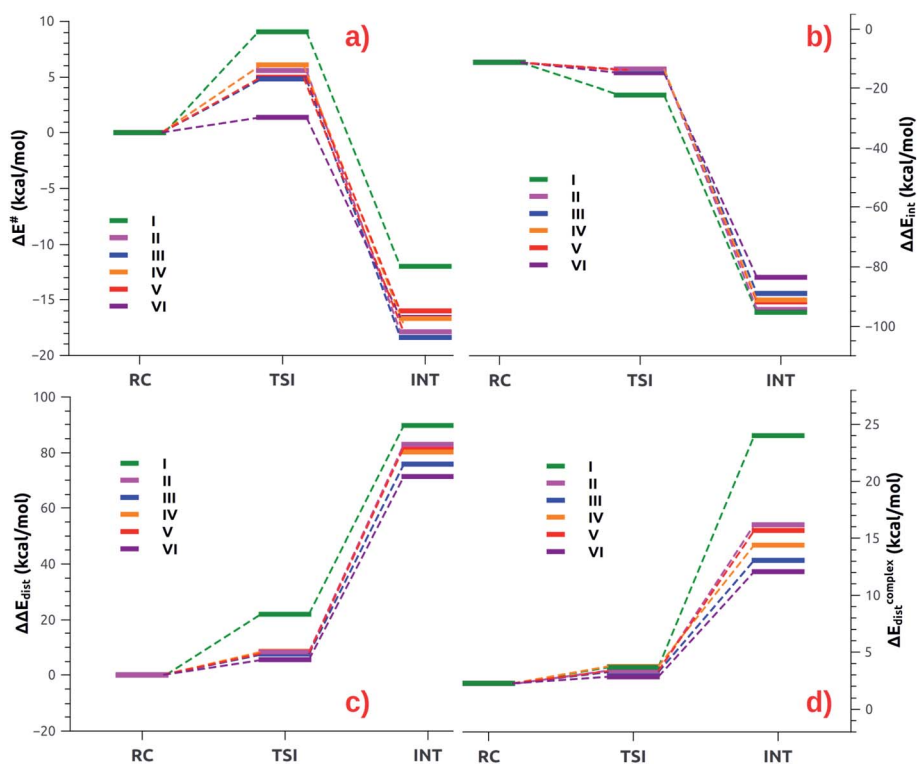
Fig. 6 (a) ASM diagrams for the electronic energy variation ( \Delta E^\ddagger ) along the reaction path connecting RC, TSI and INT structures for complexes [\text{Bu}_3\text{PAuI}] – [\text{Bu}_3\text{PAuVI}] . (b) ASM diagrams for the variation of the interaction energy stabilization ( \Delta\Delta E_{\text{int}} ) along the reaction path connecting RC, TSI and INT structures for complexes [\text{Bu}_3\text{PAuI}] – [\text{Bu}_3\text{PAuVI}] . (c) ASM diagrams for the overall variation of the distortion energy penalty ( \Delta\Delta E_{\text{dist}} ) along the reaction path connecting RC, TSI and INT structures for complexes [\text{Bu}_3\text{PAuI}] – [\text{Bu}_3\text{PAuVI}] . (d) ASM diagrams for the penalty due to the distortion of the complex ( \Delta E_{\text{dist}}^{\text{complex}} ) along the reaction path connecting RC, TSI and INT structures for complexes [\text{Bu}_3\text{PAuI}] – [\text{Bu}_3\text{PAuVI}] . Results for [\text{Bu}_3\text{PAuI}] and [\text{Bu}_3\text{PAuII}] have been taken from ref. 33 and 45, respectively.
