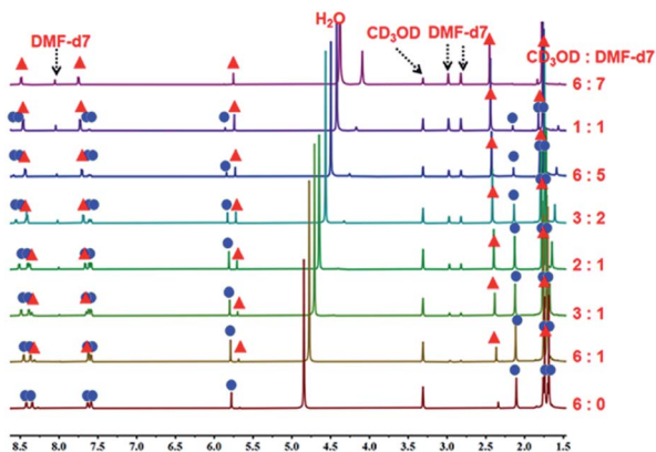
Fig. 6 The ^1\text{H} NMR spectra of metalla[2]catenane 3b (500 MHz, ppm) in \text{CD}_3\text{OD} (20.0 mmol), showing the transformation of 3b into the metallamacrocyclic 3a upon addition of \text{DMF-d}_7 .
