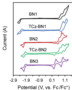
Fig. 4 Cyclic voltammograms (CV) for all compounds. The CV curves were measured at room temperature with 0.1 M solution of [n\text{-Bu}_4\text{N}] \text{PF}_6 in dichloromethane for the oxidation and reduction scan (vs. \text{Fc}/\text{Fc}^+ ).
