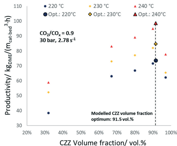
Fig. 6 Comparison of the experimental DME productivity in the run-in period and the model-optimized CZZ/FER volume ratio of 91.5/8.5 at CO 2 /CO x = 0.9, 30 bar, 2.78 s -1 and three different temperatures.
