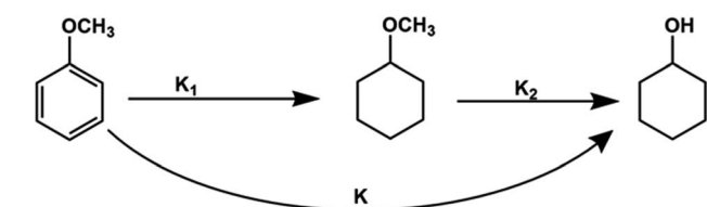
Fig. 6 Reaction mechanism and pathways of anisole hydrogenation over Ni_5Co_5 -AC.
