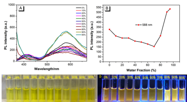
Fig. 1 (A) Fluorescence spectra of the fluorescent probe ( 2.00 \times 10^{-5} mol L^{-1} ) at different water contents ( \lambda_{ex} = 350 nm) in THF. (B) The effect of water volume fraction on the fluorescence probe at 588 nm. (C) Photographs of the fluorescent probes in THF solution containing different water components under natural light. (D) Photographs of the fluorescent probes in THF solution containing different water components under 365 nm UV light.
