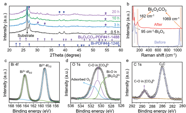
Fig. 2 (a) XRD patterns of VS- \text{Bi}_2\text{O}_3 electrolyzing the \text{CO}_2\text{RR} at 100 \text{mA cm}^{-2} after 0.5, 3, 10 and 20 h, respectively. \text{Bi}_2\text{O}_2\text{CO}_3 and Bi were formed and maintained during the \text{CO}_2\text{RR} . (b) Raman spectra of VS- \text{Bi}_2\text{O}_3 before (blue line) and after (red line) the \text{CO}_2\text{RR} for 3 h. \text{Bi}_2\text{O}_2\text{CO}_3 (orange shadow) is formed in the electrolytic process. (c–e) Bi 4f, O 1s and C 1s XPS spectra, respectively, of the post-electrolysis VS- \text{Bi}_2\text{O}_3 (at 100 \text{mA cm}^{-2} for 24 h), demonstrating the existence of \text{Bi}_2\text{O}_2\text{CO}_3 .
