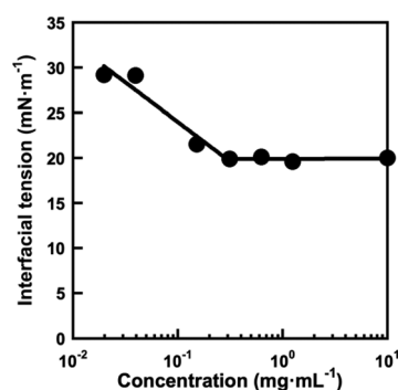
Fig. 4 Effect of P(OEGMA-co-MEO 2 MA)- b -PMPC concentration on the interfacial tension of a water–chloroform interface at 25 °C. The interfacial tension was measured using the pendant drop technique with a contact angle meter.
