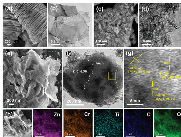
Fig. 3 (a) SEM image of multi-layered \text{Ti}_3\text{C}_2\text{T}_x nanosheets. (b) TEM image of exfoliated few-layered \text{Ti}_3\text{C}_2\text{T}_x nanosheets. (c) SEM image and (d) TEM image of collectively-grown translucent nanoflakes of pristine ZnCr-LDH, respectively. (e) SEM image and (f) TEM image of ZnCr-LDH grown on \text{Ti}_3\text{C}_2\text{T}_x , respectively. (g) HRTEM image of ZCTC25. (h) SEM elemental mapping images of ZCTC25.
