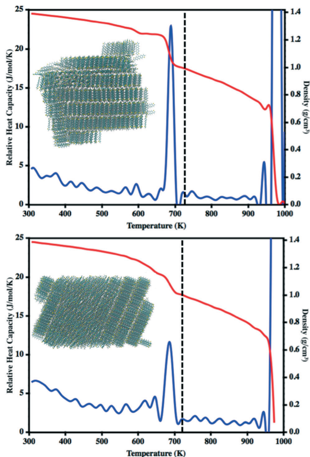
Fig. 9 Relative heat capacity (blue) and simulation box density (red) of anti ADT (top) and syn ADT (bottom) as the recrystallized system is heated from 300 K to 1000 K. The experimental melting points of the anti ADT (725 K) and syn ADT (720 K) are highlighted with dashed, black lines. The insets show the respective initial system morphologies prior to reheating.
