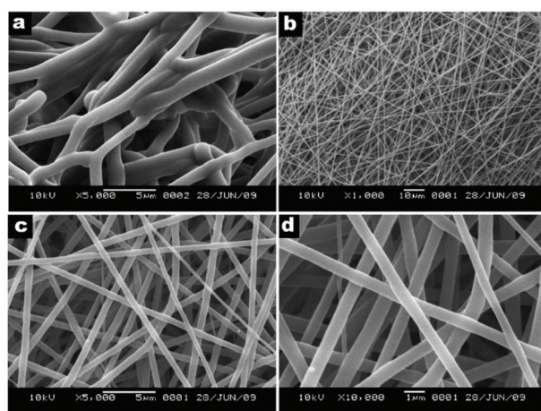
Fig. 4 SEM images of (a) PAN fibers electrospun at 24 °C, and (b–d) Acyclovir-loaded PAN fibers electrospun at 80 °C with different magnifications. Reproduced from ref. 73 with permission from Elsevier.
