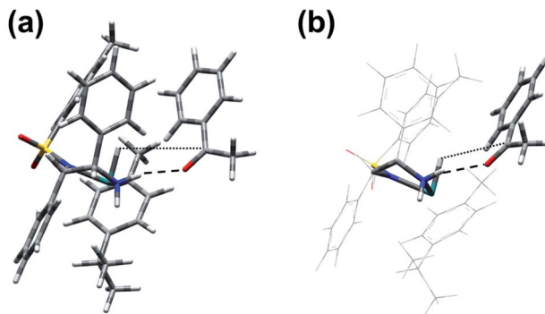
Fig. 8 (a) Pre-organisation of the [\text{Ru}(\text{p-cymene})(\text{S},\text{S-TsDPEN-H})]/\text{acetophenone} assembly with \text{CO}\cdots\text{H}_2\text{N} H-bonding (denoted by the dashed line), the initial stage of the catalytic cycle. Note that the vector defined by hydride H and carbonyl C atoms points towards one of the enantiotopic faces of the ketone. (b) Simplified scheme to highlight bonding interactions between catalyst diamine and substrate carbonyl (Fig. S16, PDB13†).
