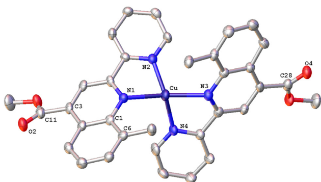
Fig. 7 Molecular structure of the cation of complex [\text{Cu}(8\text{-Mepqame})_2][\text{PF}_6] (2(7\text{-C}_5\text{H}_{12})) \cdot \text{CHCl}_3 ; ellipsoids are plotted at the 50% probability level. H atoms, except those in the COOH groups, and the co-crystallized solvents are omitted for clarity.
