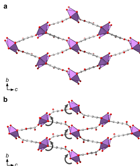
Fig. 5 (a) The structure of as-synthesized 1 EtOH as determined by 3DED viewed along a showing a similar pore shape as 1 MeOH. (b) The structure of partially activated 1 EtOH(stored) as viewed along a , showing an altered pore shape, resulting in a 24% decrease in unit cell volume (1181(10) Å 3 to 891(8) Å 3 ) upon loss of solvent. Semicircular arrows are drawn to illustrate the concerted rotation of the IBUs in the structure. The ethanol carbon atoms and hydrogen atoms are omitted for clarity.
