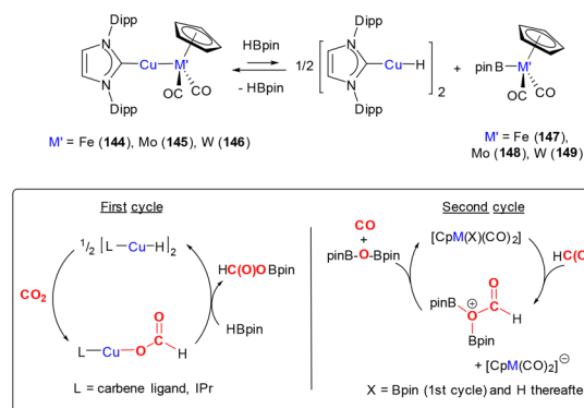
Scheme 43 Mechanism for the 2-electron reduction of CO 2 to CO catalysed by heterobimetallic complexes [(NHC)Cu–ML n ] {ML n = [FeCp(CO) 2 ], [WCp(CO) 3 ], [MoCp(CO) 3 ]}. X = Bpin (1st cycle) and H thereafter
