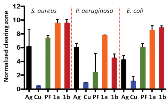
Fig. 13 Efficacy of PF based compounds: Normalized zones of growth inhibition utilizing compound impregnated disks [Ag = \text{AgNO}_3 , PF = proflavine, Cu = CuCl, 1a = \text{PF}\cdot\text{CuCl} , 1b = \text{PF}\cdot\text{AgNO}_3 ]. Reproduced from ref. 68 with permission from the Royal Society of Chemistry.
