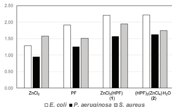
Fig. 15 Fold antimicrobial activity of proflavine, \text{ZnCl}_3(\text{HPF}) and (\text{HPF})_2[\text{ZnCl}_4]\cdot\text{H}_2\text{O} compared to the activity of \text{AgNO}_3 (the value of 1.00 is equal efficacy as silver nitrate). Reproduced from ref. 69 with permission from the Royal Society of Chemistry.
