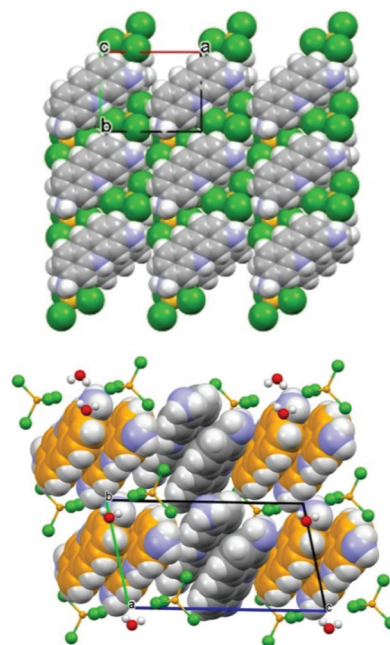
Fig. 14 (Top) Projection in the ab -plane of crystalline \text{ZnCl}_3(\text{HPF}) in which the molecules are arranged in piles along the c -axis direction. (Bottom) Projection down the crystallographic b -axis of crystalline [\text{HPF}]_2[\text{ZnCl}_4]\cdot\text{H}_2\text{O} , showing the herring-bone pattern of \text{HPF}^+ cationic pairs. Reproduced from ref. 69 with permission from the Royal Society of Chemistry.
