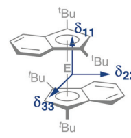
Fig. 4 Schematic depiction of the principal axes of the chemical shift tensors \delta_{11} , \delta_{22} and \delta_{33} in 2a–c .
