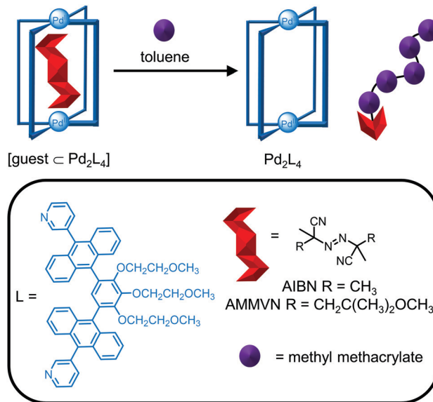
Fig. 15 Stabilisation of radical initiators within a \text{Pd}_2\text{L}_4 cage reported by Yoshizawa and co-workers. Subsequent release from the cage in toluene restored the reactivity of the radical initiator for the polymerisation of methyl methacrylate.
