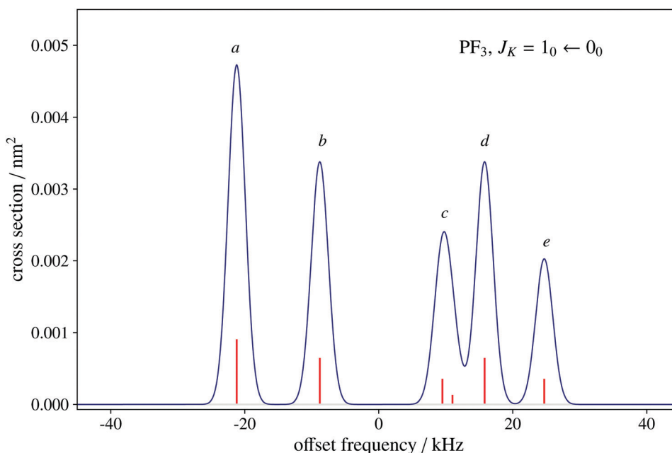
Fig. 1 Spectral simulation of the J_K = 1_0 \leftarrow 0_0 rotational transition of PF 3 as can be observed using a pulsed-jet Ball–Flygare Fourier-transform microwave spectrometer. The x -axis scale is expressed as the offset with respect to the unperturbed frequency value of 15637.959 MHz. The y -axis scale indicates the absorption cross section computed at 2 K, the typical rotational temperature obtained in a supersonic-jet cooled sample. The hyperfine components are labelled as F'_1, F' \leftarrow F_1, F . (a) 1.5, 3 \leftarrow 0.5, 2 ; (b) 1.5, 2 \leftarrow 0.5, 1 and 1.5, 2 \leftarrow 0.5, 2 ; (c) 1.5, 1 \leftarrow 0.5, 1 , 1.5, 1 \leftarrow 0.5, 2 , and 1.5, 0 \leftarrow 0.5, 1 ; (d) 1.5, 2 \leftarrow 0.5, 1 and 1.5, 2 \leftarrow 0.5, 2 ; (e) 1.5, 1 \leftarrow 0.5, 1 and 1.5, 1 \leftarrow 0.5, 2 . The I_{\text{tot}} for K = 0 is always 1.5 because of spin statistics.
