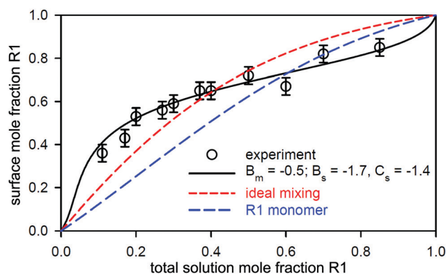
Fig. 12 Variation in surface composition with solution composition for a 1 m R1/R2 mixture. The black line is the best PPA description for the parameters shown (in units of RT ), ideal surface mixing is shown as a short dashed red line, and the long dashed blue line is the associated monomer composition. Redrawn from Liley et al. 113
