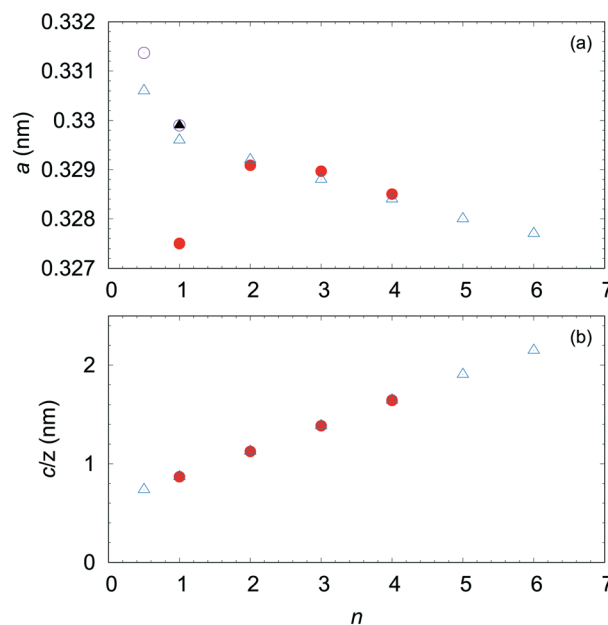
Fig. 18 (a) Lattice parameter a and (b) layer width c/Z of homologous compounds \text{InGaO}_3(\text{ZnO})_n as function of n . Open triangle symbols represent lattice constants estimated from the polycrystalline sample. 23 Solid triangles represent small single crystal obtained from high pressure (2 GPa). 45 Open circle symbols represent estimates from single crystals grown by the OFZ method. 55 Solid circles represent estimates from small single crystals. 46,48,49
