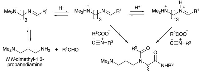
Fig. 1 The effect of adding 1 equivalent of HCl (or p -TsOH) to the Ugi reaction based on N,N -dimethyl-1,3-propanediamine.
