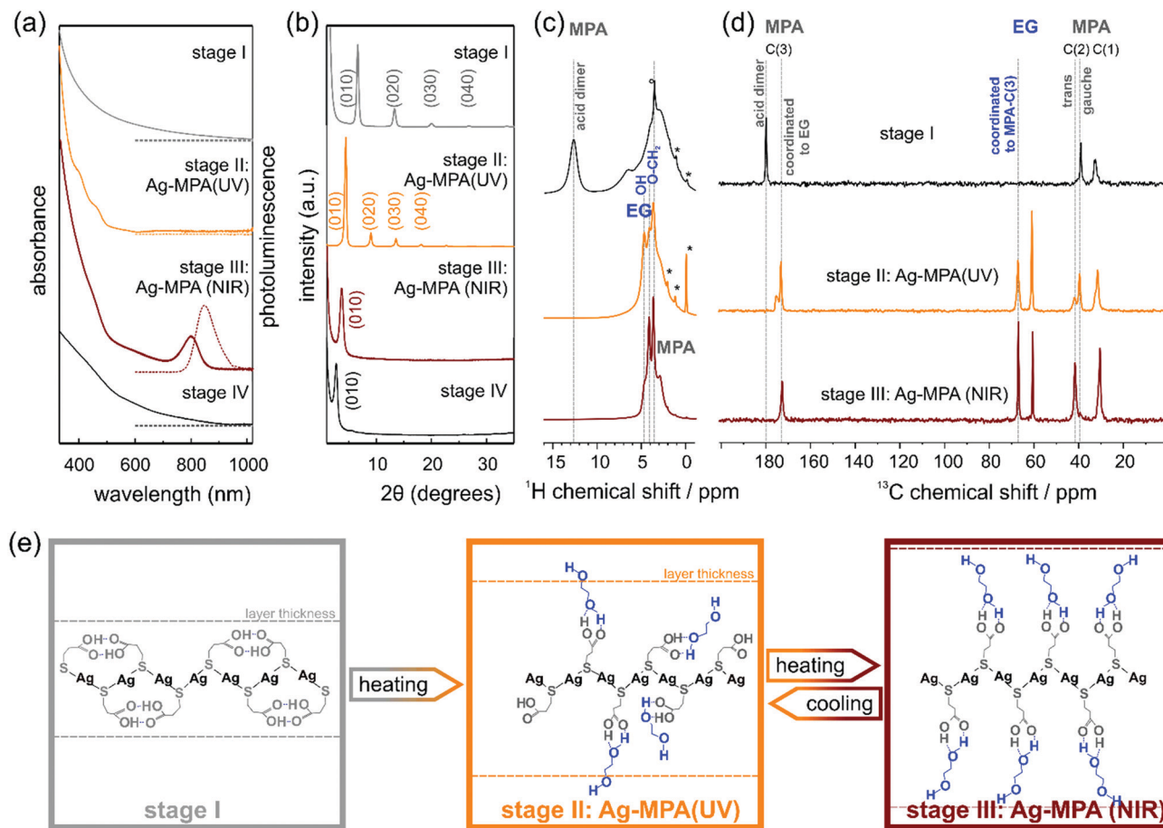
Fig. 1 (a) Absorption spectra (solid lines) and photoluminescence spectra (dash lines), (excited by 380 nm); (b) PXRD patterns; (c) ^1\text{H} MAS NMR spectra (asterisk marked the contaminated with silicon grease and residual solvent); (d) ^{13}\text{C} NMR spectra; (e) the scheme of structures at different reaction stages.
