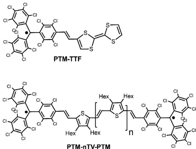
Scheme 6 Chemical structures of the Veciana and Rovira compounds with diradical character ( PTM- n TV-PTM , with n = 1-6 ) and the PTM tetrathiafulvalene neutral radical, PTM-TTF .
