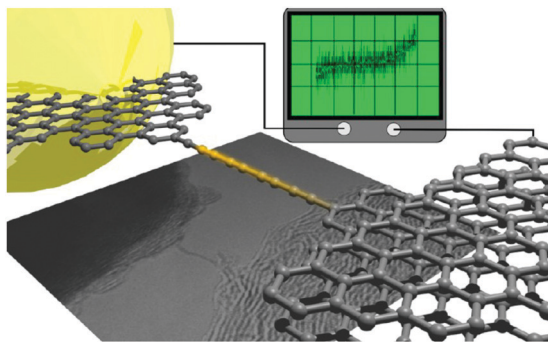
Fig. 12 Schematic representation and TEM image of a conducting monoatomic carbon chain between graphene electrodes and an I - V trace of the device. Reproduced from ref. 125 with permission from the American Chemical Society.
