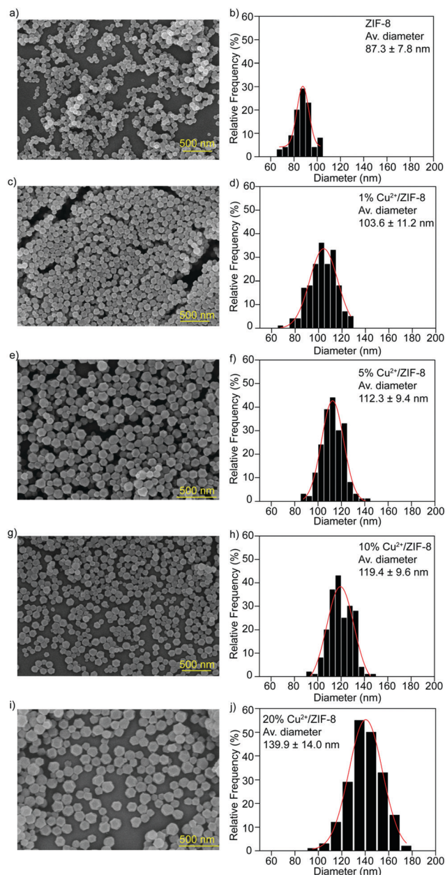
Fig. 3 SEM images and size distributions of (a and b) ZIF-8, (c and d) 1% Cu 2+ /ZIF-8, (e and f) 5% Cu 2+ /ZIF-8, (g and h) 10% Cu 2+ /ZIF-8, and (i and j) 20% Cu 2+ /ZIF-8. Scale bars: 500 nm.
