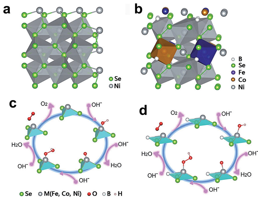
Fig. 14 (a and b) Schematic illustration of NiSe 2 and Fe 5 Co 4 Ni 20 Se 36 B x crystal structures, and (c and d) proposed OER mechanisms for pyrite selenides before and after B dopant incorporation. 163 Reproduced from ref. 163 with permission, © 2019 American Chemical Society.
