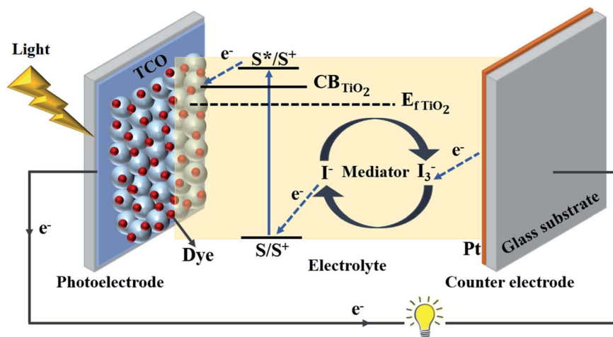
Fig. 2 Schematic illustration representing device structure and working principle of a dye-sensitized solar cell. CB = conduction band, E_{fTiO_2} = fermi level of TiO 2 , S = ground state of dye sensitizer molecule, S* = excited state of dye sensitizer molecule, S + = oxidized dye, S + = charge separation, I - = iodide ion and I 3 - = triiodide ion.
