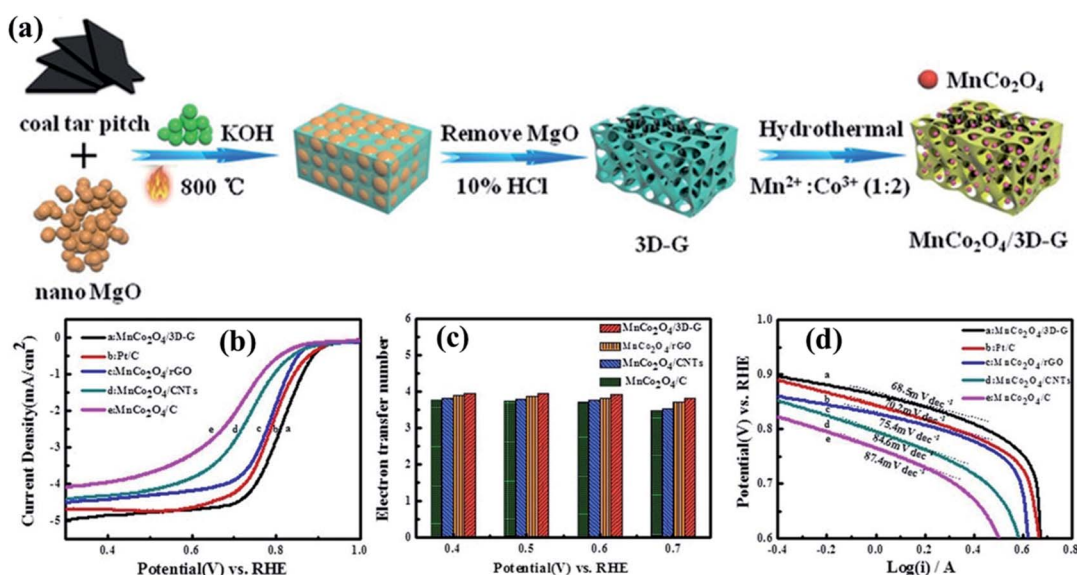
Fig. 8 (a) The synthesis route to the \text{MnCo}_2\text{O}_4 /3D-G catalyst. (b) LSV curves of the different catalysts. (c) Electron transfer number per oxygen molecule of the different catalysts at different potentials. (d) Tafel slopes of the electrode assemblies fabricated with different catalysts. Reproduced with permission from ref. 185. Copyright © 2018 Wiley-VCH Verlag GmbH & Co. KGaA, Weinheim.
