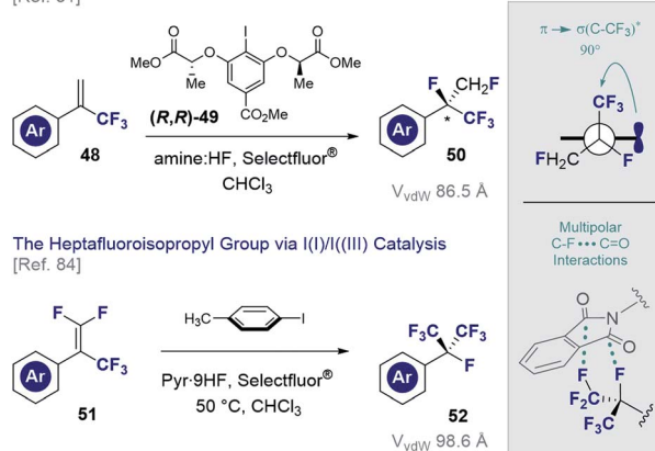
Fig. 12 Generating fluorinated surrogates of the isopropyl group via I(I)/I(III) catalysis.
