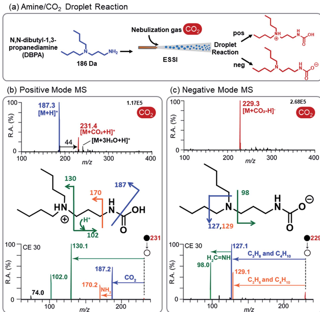
Fig. 1 DBPA/CO 2 droplet reaction by adding CO 2 in the gas phase (a) Droplet reaction of amine/CO 2 conducted by ESI. (b) Positive and (c) negative mode mass spectra and MS/MS spectra showing fragmentation of protonated and deprotonated DBPA carbamic acid.
