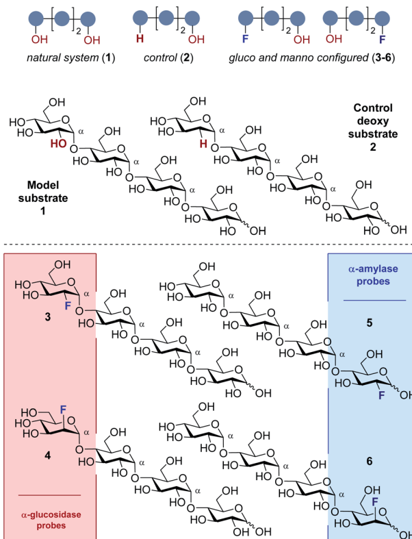
Fig. 3 The maltotetraose probe set for this study.
