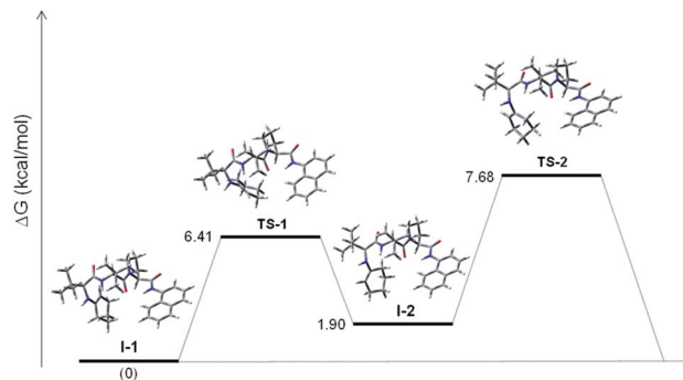
Fig. 1 Energy profile of the interconversion of 6c .
