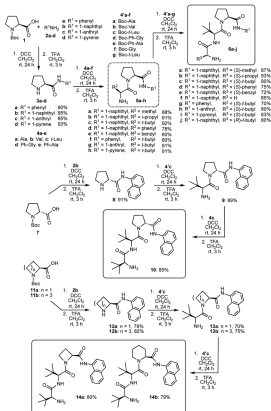
Scheme 2 Preparation of di- and tripeptide organocatalysts.
