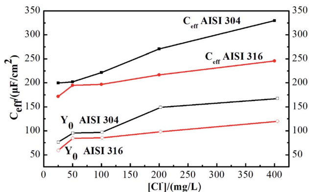
Fig. 4 Admittance ( Y_0 ) and calculated effective capacitance ( C_{\text{eff}} ) of AISI 304 and AISI 316 at different chloride concentration.
