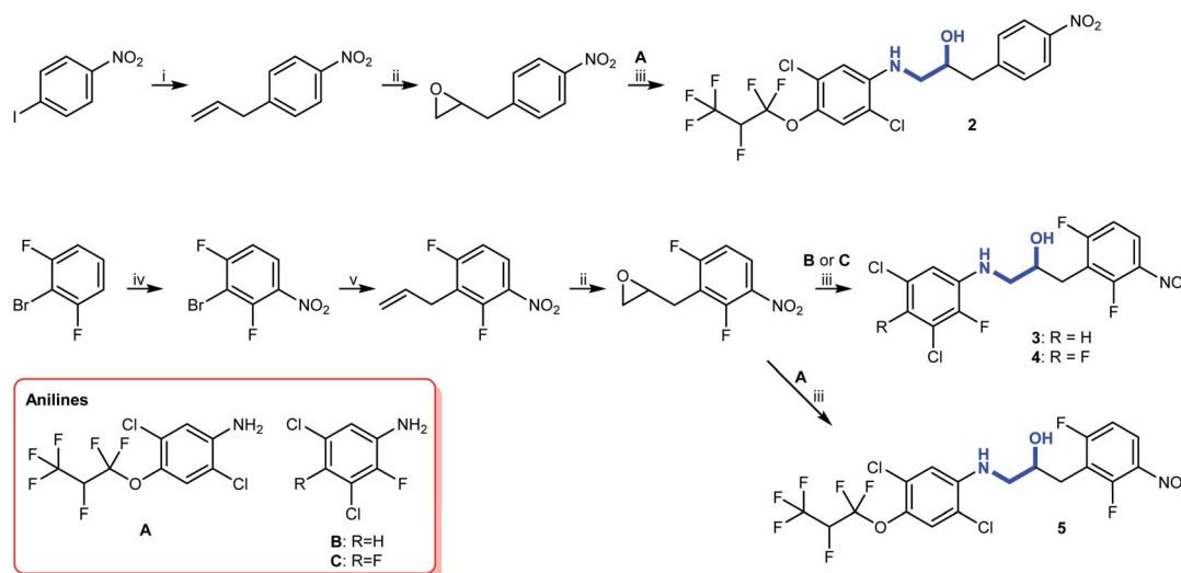
Scheme 3 Synthesis of aminols 2–5. Reagents and conditions: (i) Pd(PPh 3 ) 4 , CsF, AllylBpin, THF, reflux; 27 (ii) m CPBA, DCM, rt; (iii) 5 M LPDE, 40 °C; (iv) H 2 SO 4 , HNO 3 , 0 °C; (v) Pd(PPh 3 ) 4 , Bu 3 SnAllyl, DMF, 110 °C.
